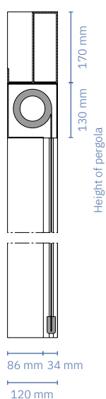
Section view A-A
